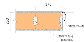
- BONDING AT THE DOOR REVEAL, 1ST ROW OF BRICKWORK
