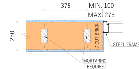
- BONDING AT THE DOOR REVEAL, 2ND ROW OF BRICKWORK
