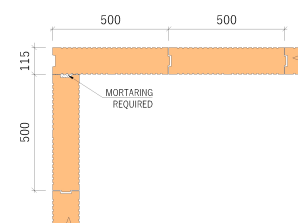
- CORNER BONDING, 2ND ROW OF BRICKWORK
