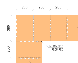
- CORNER BONDING, 2ND ROW OF BRICKWORK
