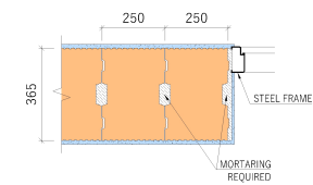
- BONDING AT THE DOOR REVEAL, 1ST ROW OF BRICKWORK
