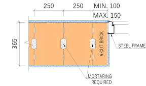
- BONDING AT THE DOOR REVEAL, 2ND ROW OF BRICKWORK
